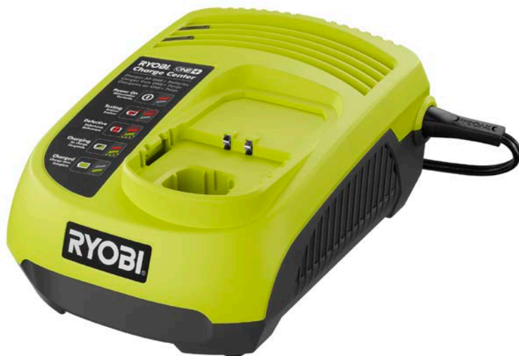
Photo 1 Ryobi Model P113 Dual Chemistry Charger
